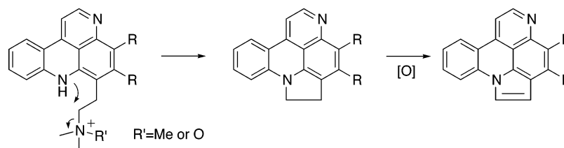
Figure 3. Proposed mechanism for the formation of arnoamine A ( 24 )/cycloderictin ( 19 ).
